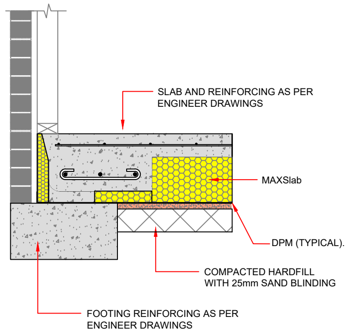
MAXSlab BRICK TO FOOTING DETAIL
