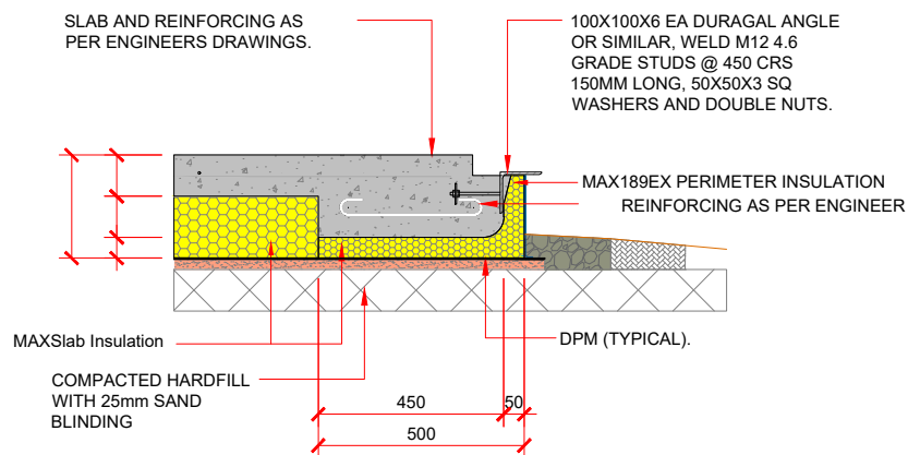
MAXSLAB HEAVY DOOR / WINDOW SUPPORT DETAIL
