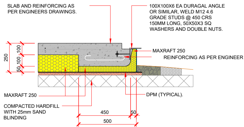
MAXSLAB HEAVY DOOR / WINDOW SUPPORT DETAIL
