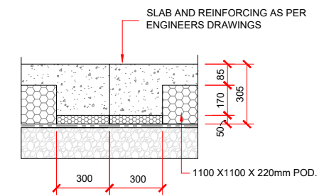
FREE JOINT / CONTROL JOINT DETAIL
