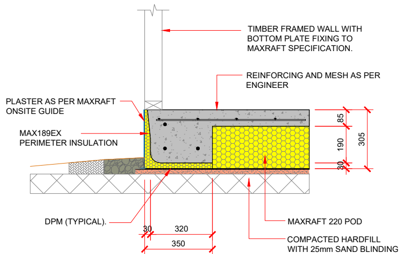
MAX85 Perimeter Detail
