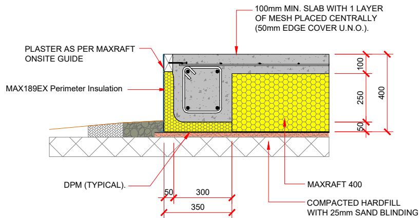
MAXRAFT 400 WANZ BAR FIXING DETAIL
