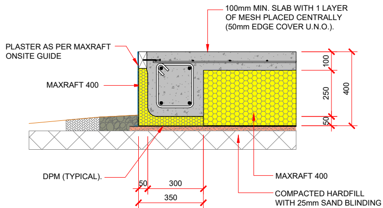
MAXRAFT 400 WANZ BAR FIXING DETAIL
