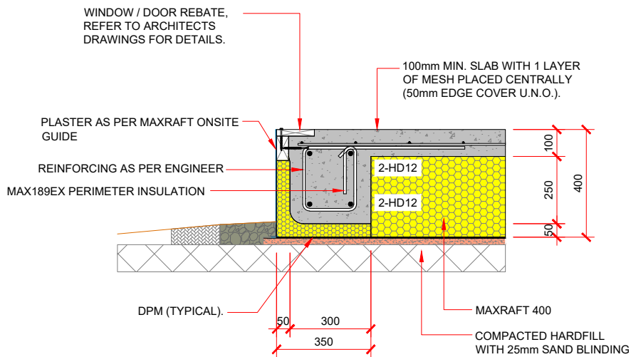
MAXRAFT 400MM REBATE / WANZ BAR FIXING DETAIL
