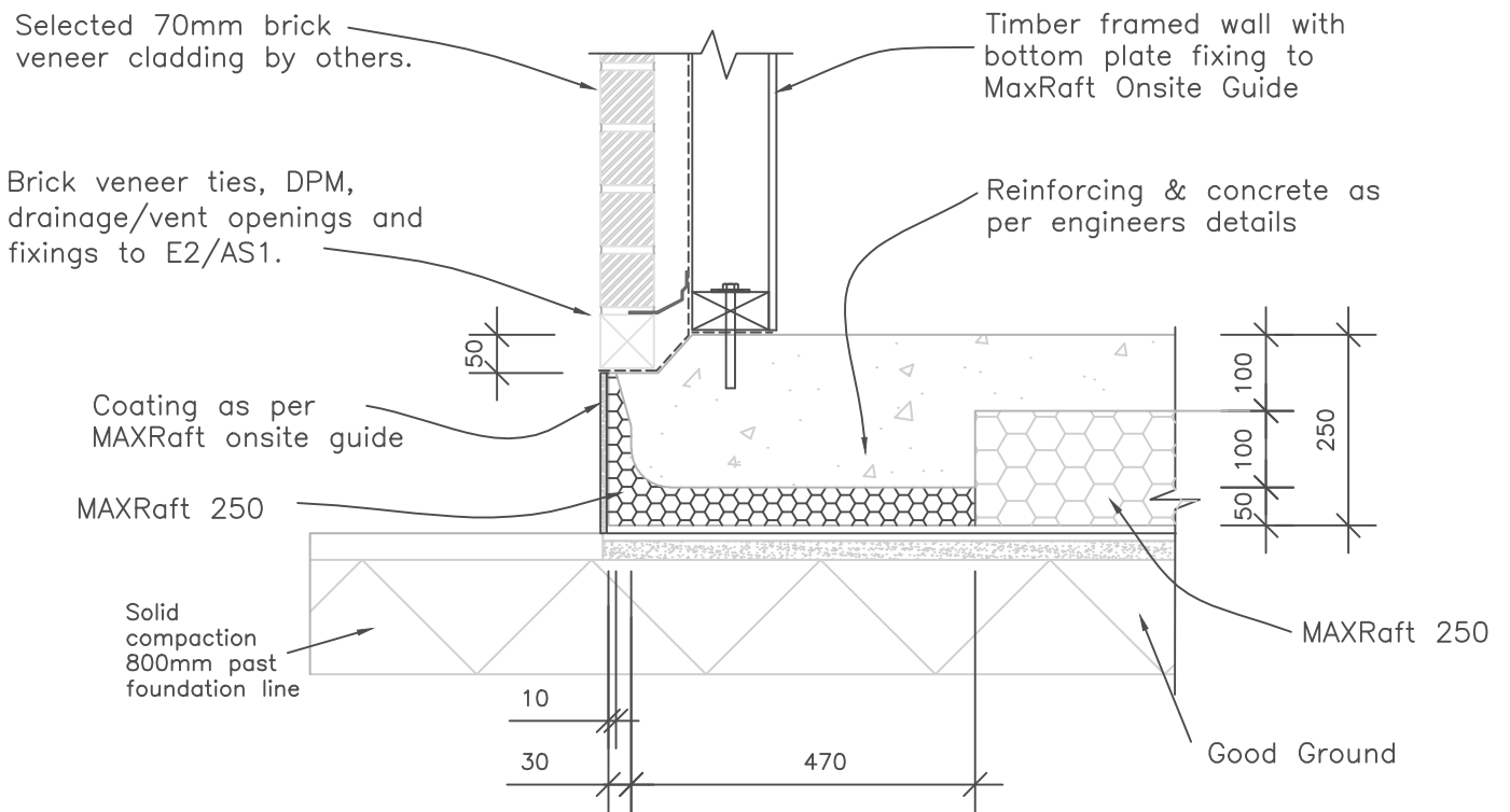
MAXRaft© 250 - 70mm Brick Veneer
