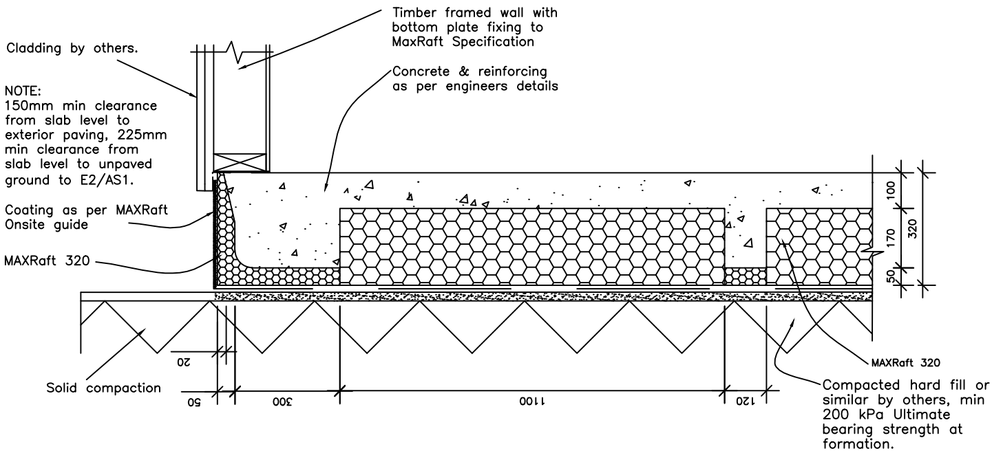
MAXRaft© 320 / 400 – Timber Frame with Lightweight cladding
