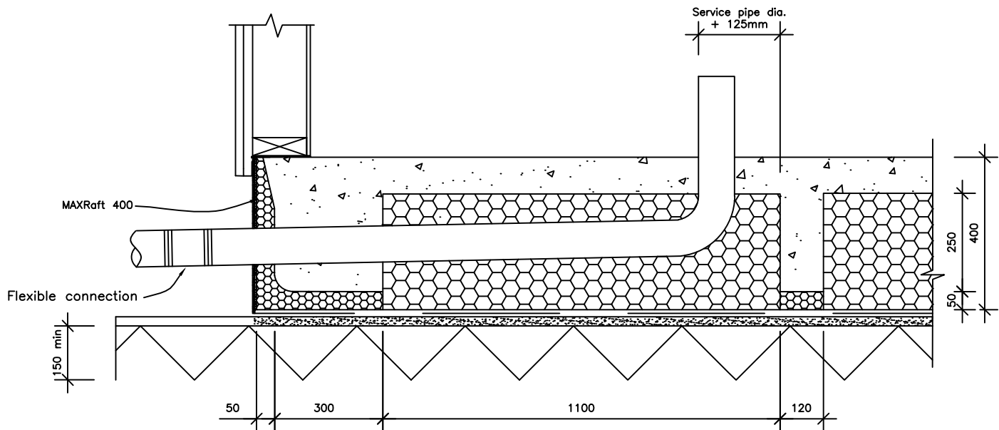
MAXRaft© 320 / 400 – Typical pipe penetration Detail
