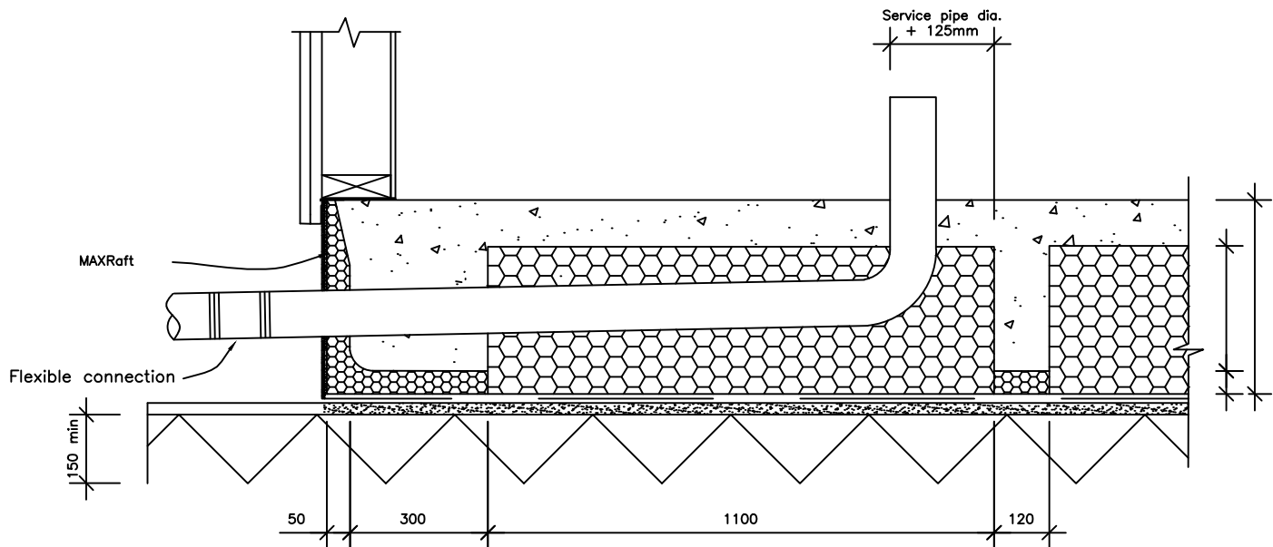
MAXRaft© Typical pipe penetration Detail
