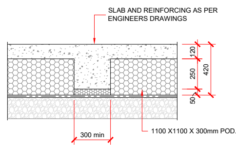
INTERNAL FOOTING DETAIL
