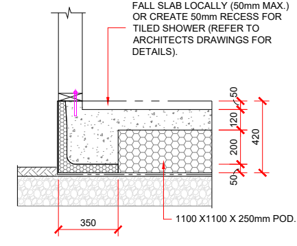
SHOWER RECESS DETAIL - 140mm FRAMING.
