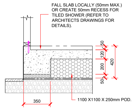
SHOWER RECESS DETAIL - 90mm FRAMING.
