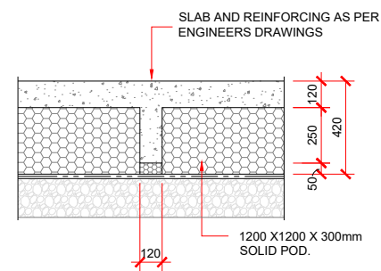
INTERNAL RIB DETAIL
