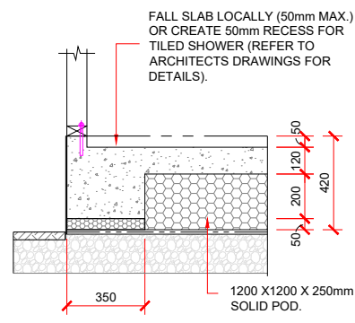
SHOWER RECESS DETAIL - 90mm FRAMING.
