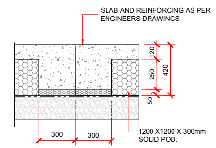
FREE JOINT / CONTROL JOINT DETAIL
