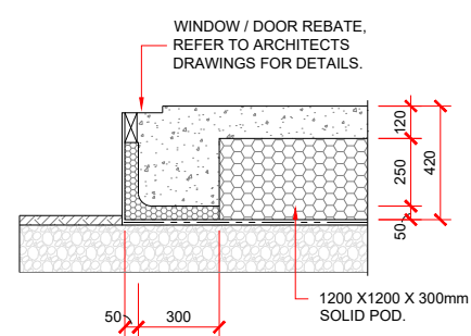
JOINERY REBATE DETAIL
