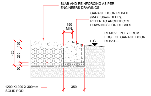
GARAGE DOOR REBATE DETAIL
