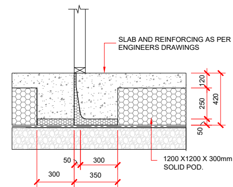
BRICK / STONE VENEER REBATE DETAIL
