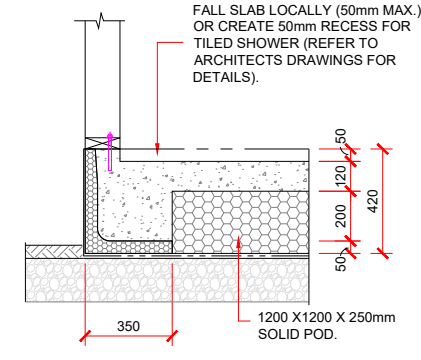
SHOWER RECESS DETAIL - 140mm FRAMING.
