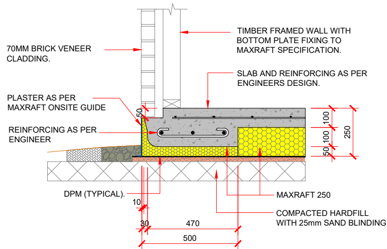
EXTERNAL FOOTING DETAIL
