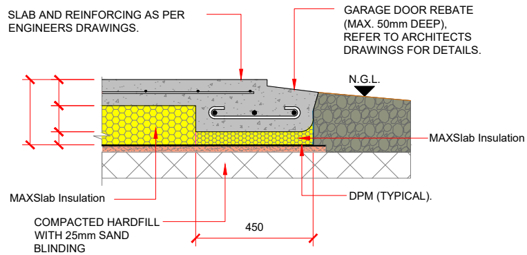
GARAGE DOOR REBATE DETAIL
