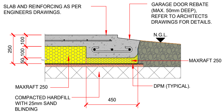
GARAGE DOOR REBATE DETAIL
