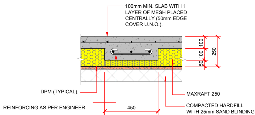
MAXSLAB INTERNAL FOOTING DETAIL
