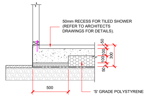
SHOWER RECESS DETAIL - 90mm FRAMING.
