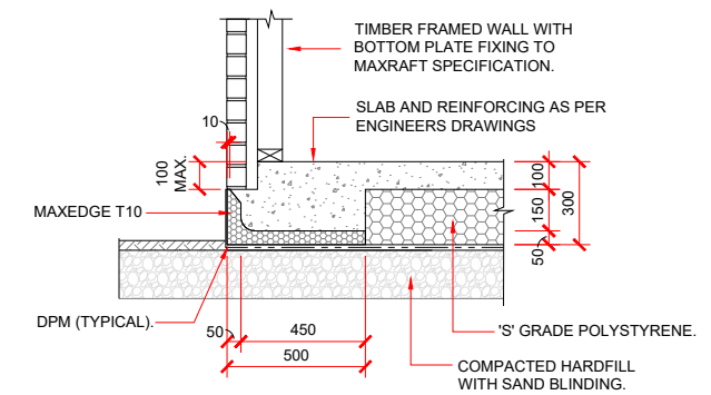
BRICK / STONE VENEER REBATE DETAIL
