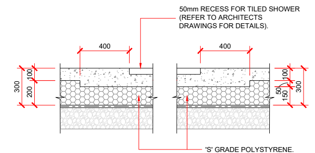
SHOWER RECESS DETAIL.
