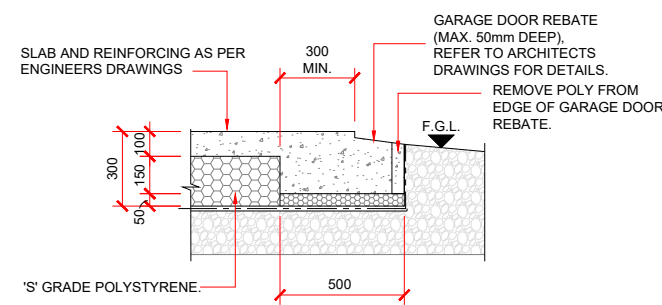
GARAGE DOOR REBATE DETAIL
