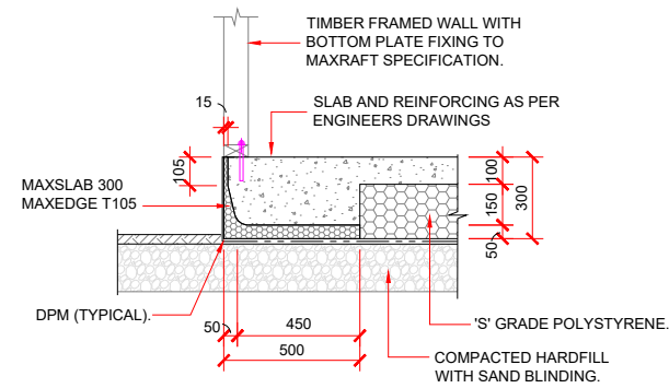
EXTERNAL FOOTING DETAIL MAXEDGE T105 - 90mm FRAMING
