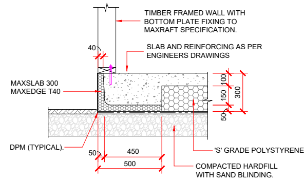
EXTERNAL FOOTING DETAIL MAXEDGE T40 - 140mm FRAMING
