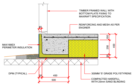
EXTERNAL FOOTING DETAIL
